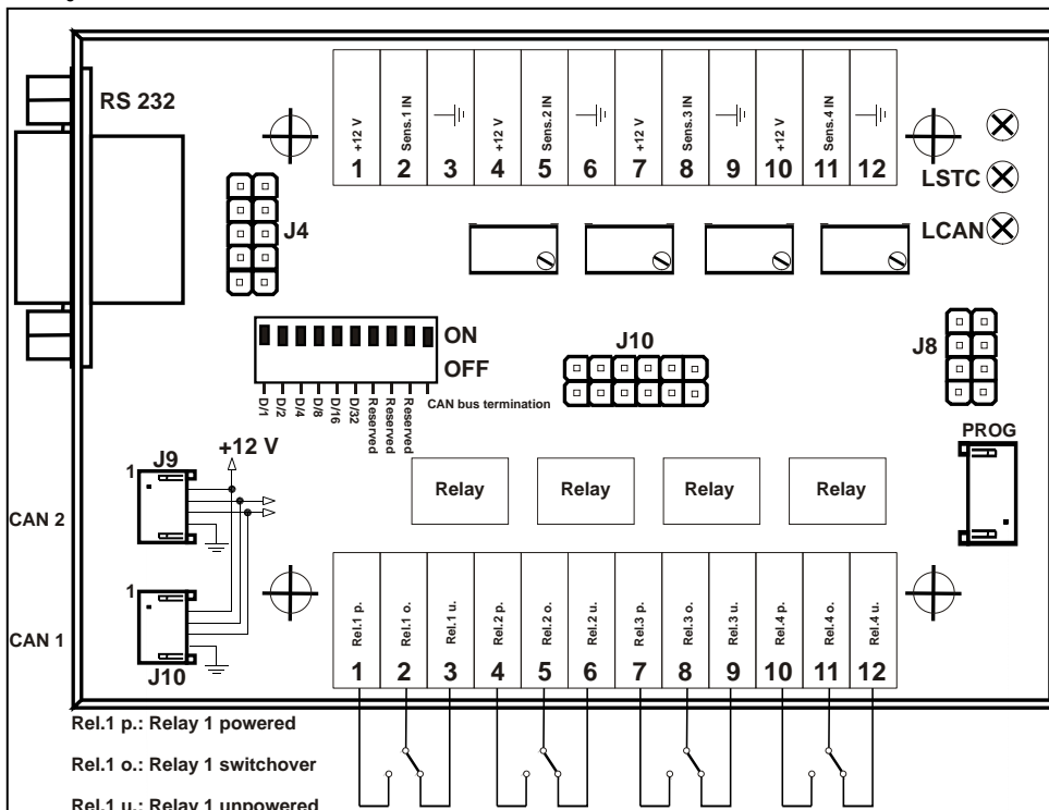
Fig. 2: Schematic diagram
