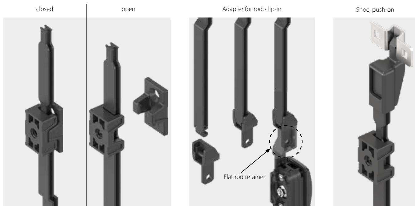
Rod guide Polyamide GF black 1190-30-01 for weld stud M6x10 and flat nut M6
