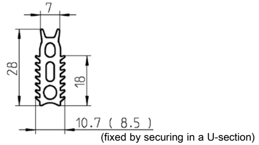
Fire protection sealing Profile silicon solid material 50° ±5° Shore A graphite grey
